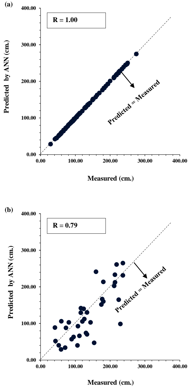
Figure 31. Predicted vs. measured water levels in piezometer 42L of Control 19G (a) Training data; (b) Testing data
