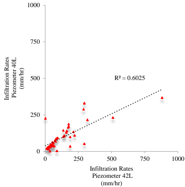
Figure 19. Gallery permeability rates comparison of PICP 19H (a) Piezometer 41L-40L (b)
