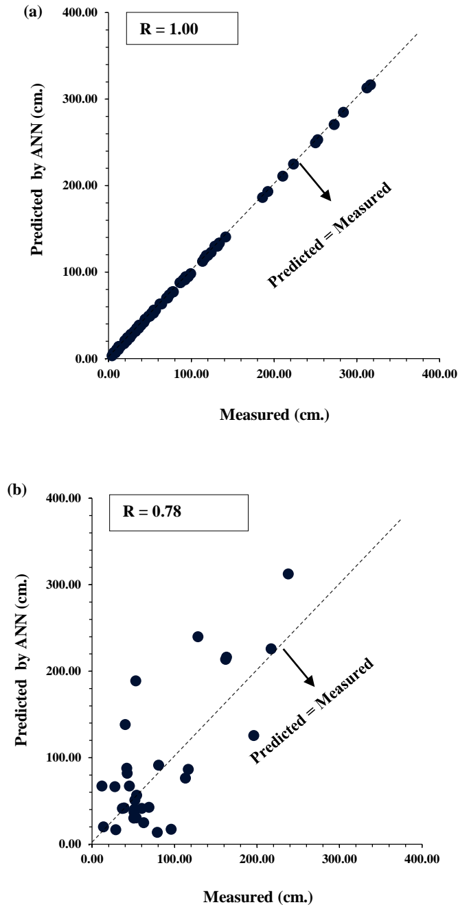
Figure 32. Predicted vs. measured water levels in piezometer 40L of Control 19H (a) Training data;
