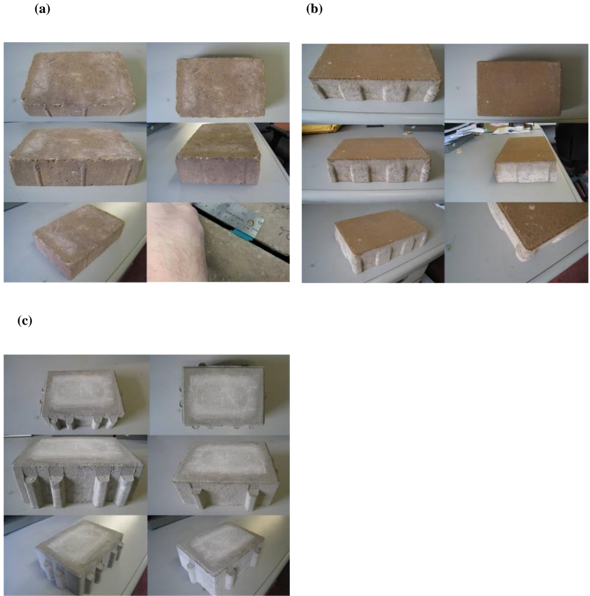
Figure 16. Paver block types (a) Coventry I® (b) Eco-Cobble® (c) Eco-Paver® (Antunes 2013)
